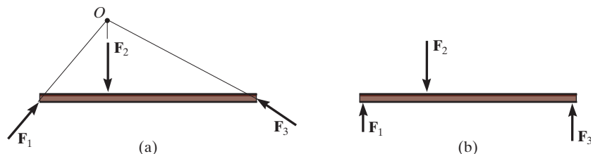
Three-force member
