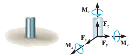
fixed support
